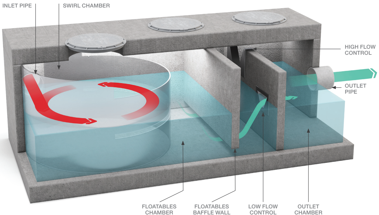
Figure 1: Vortechs™ components
